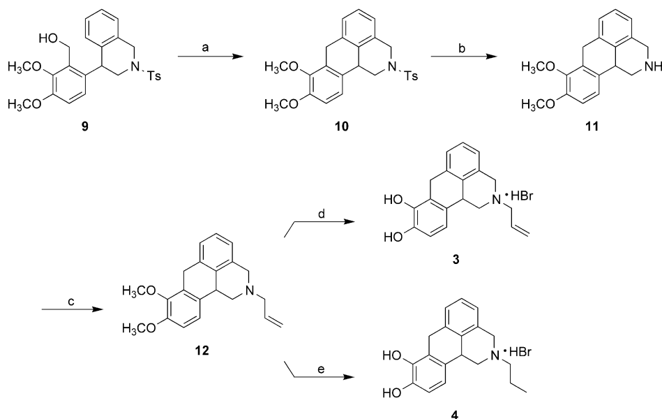
Scheme 1. Reagents and conditions: (a) concd \text{H}_2\text{SO}_4 , -20^\circ\text{C} (31%); (b) \text{Na}(\text{Hg}) , \text{Na}_2\text{HPO}_4 , \text{MeOH} (74%); (c) allyl bromide, \text{K}_2\text{CO}_3 , acetonitrile (94%); (d) \text{BBr}_3 , \text{CH}_2\text{Cl}_2 , -78^\circ\text{C} (89%); (e) (i) 10% \text{Pd/C} , ethanol; (ii) \text{BBr}_3 , \text{CH}_2\text{Cl}_2 , -78^\circ\text{C} (66%, two steps).
