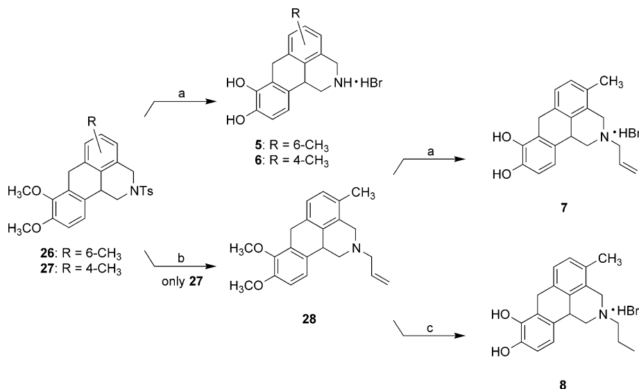
Scheme 5. Reagents and conditions: (a) (i) Na(Hg), Na 2 HPO 4 , methanol; (ii) BBr 3 , CH 2 Cl 2 , –78 °C (5: 61%, 6:73%, 7:62%); (b) (i) Na(Hg), Na 2 HPO 4 , methanol; (ii) allyl bromide, K 2 CO 3 , acetonitrile; (c) (i) 10% Pd/C, ethanol; (ii) BBr 3 , CH 2 Cl 2 , –78 °C, (59%, two steps).
