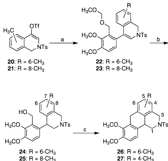
Scheme 4. Reagents and conditions: (a) 13, Pd(PPh 3 ) 4 , KBr, KOH, toluene, reflux (22: 91%, 23: 92%); (b) i. Pd/C (10%), H 2 , ethanol, ii. 3N HCl–THF (1:1) (24: 75%, 25: 79%); (c) concd H 2 SO 4 , –20 °C (26: 42%, 27: 62%).
