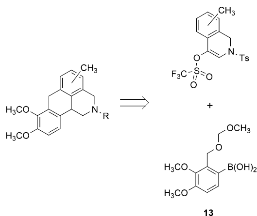
Scheme 2. Retrosynthetic analysis for methyl-substituted analogues of 2 .
