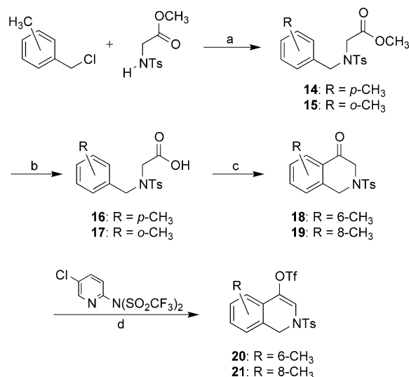
Scheme 3. Reagents and conditions: (a) \text{K}_2\text{CO}_3 , \text{NaI} , acetone, reflux (14: 76%, 15: 90%); (b) 10% \text{NaOH} (16: 85%, 17: 94%); (c) \text{SOCl}_2 , \text{AlCl}_3 , -78 \rightarrow -11^\circ\text{C} , \text{CH}_2\text{Cl}_2 (18: 70%, 19: 70%); (d) ( n - \text{BuLi} , \text{HN}(\text{iPr})_2 , \text{THF} , -78 – 0^\circ\text{C} (20: 77%, 21: 77%)).
