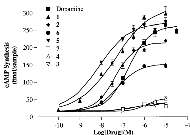
Figure 2. Functional effects of DNS and analogues at C-6-mD1 receptors. Dopamine and dihydroxidine are included for reference. Consistent with data from striatal membranes, notice the unexpected and significantly greater potency and intrinsic activity of 5 versus 6 . Stimulation of D 1 receptors by agonists was blocked by the D 1 antagonist SCH23390 (data not shown).
