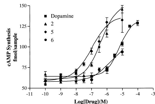
Figure 1. Functional effects of DNS and analogues at rat striatal D 1 receptors. Some agonists are not depicted because they showed minimal stimulation (see Table 3). Dopamine is included for reference. Note the significantly greater potency and intrinsic activity of 5 versus 6 . Stimulation of D 1 receptors by agonists was blocked by the D 1 antagonist SCH23390 (data not shown).
